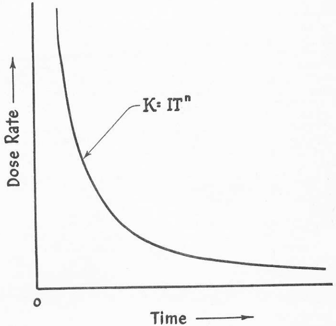
Figure 6—Multiple Decay.
