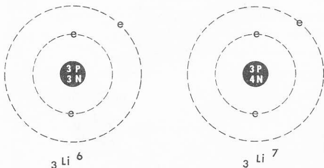
Figure 2—Diagram of Lithium Isotopes.
