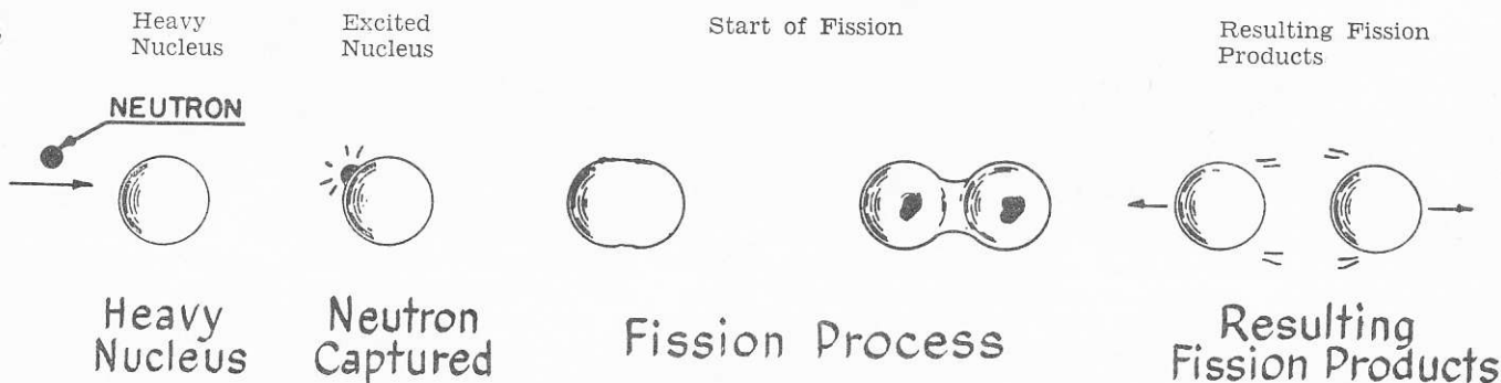
Figure 3—Fission Process.
