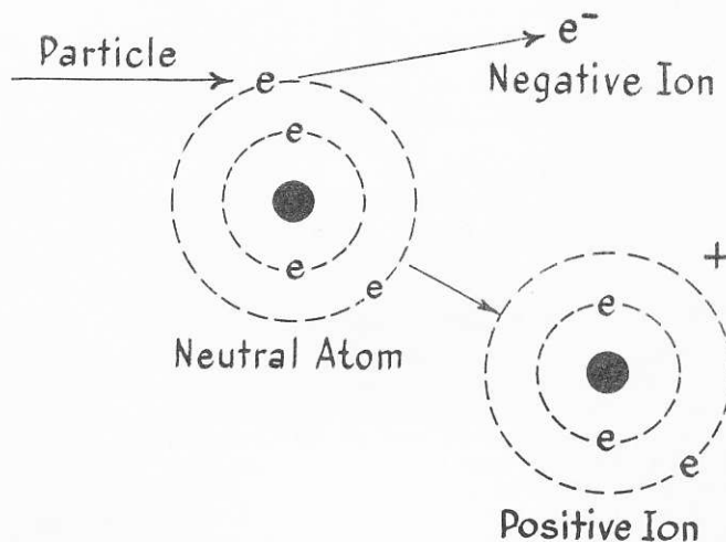
Figure 7—Ionization.
